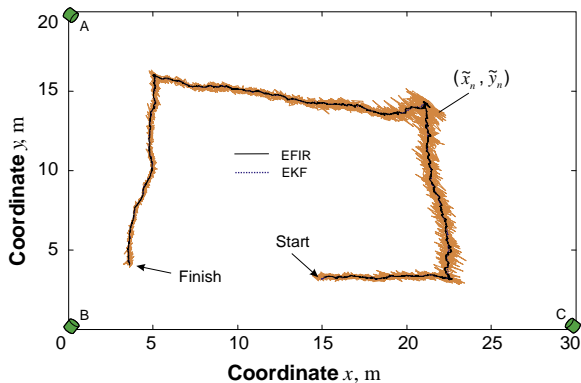
Fig. 5. Localization by (8)–(10) and extended filters of a robot traveling stepwise on a floorspace of dimensions (30 × 20) m in noisy environment. The EFIR and EKF produce consistent estimates.
